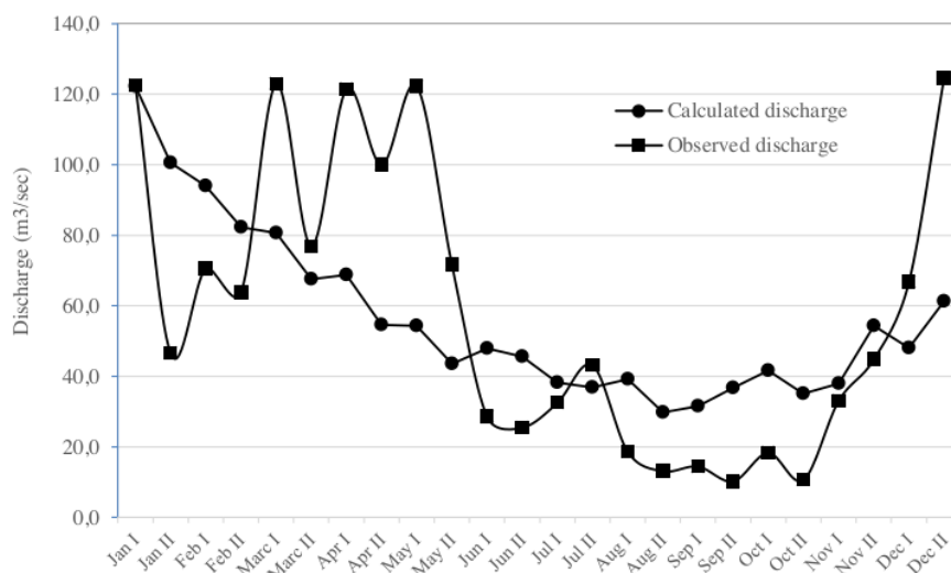
Figure 6. Calibration graph of measured and calculated data in Riam Kiwa river
