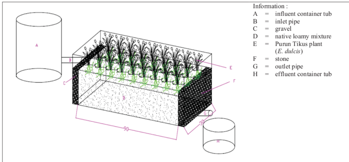
FIGURE 2. Rain garden reactor design
