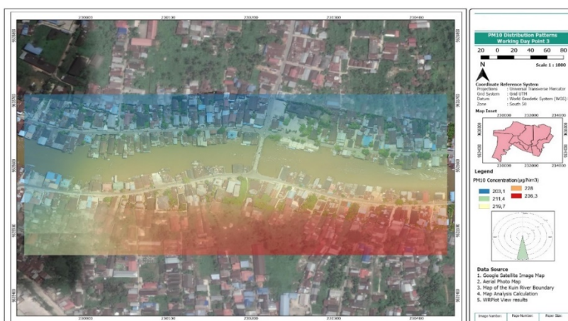
Figure 7. PM 10 dispersion patterns station III (weekdays)
