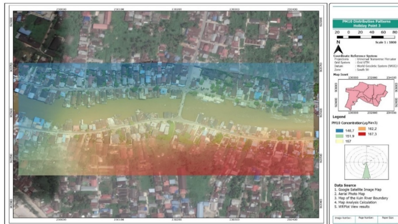
Figure 4. PM 10 dispersion patterns station III (weekend)
