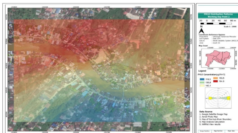
Figure 6. PM 10 dispersion patterns station II (weekdays)
