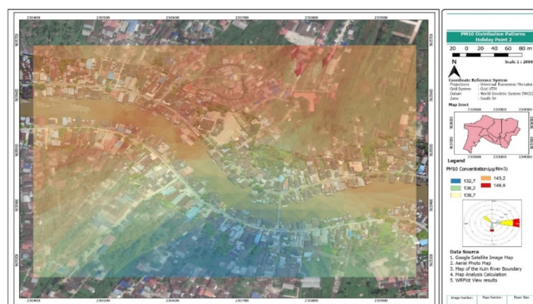
Figure 3. PM_{10} dispersion patterns station II (weekend)
