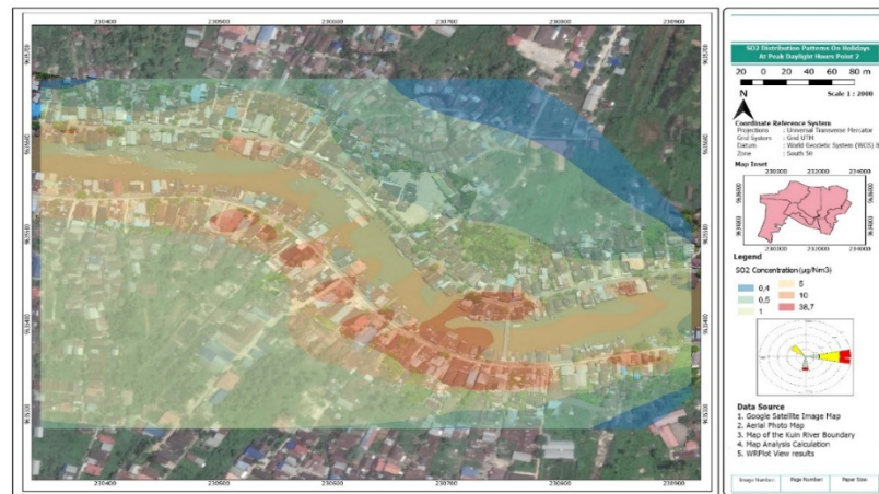
Figure 9. SO 2 dispersion patterns station II (Weekend)
