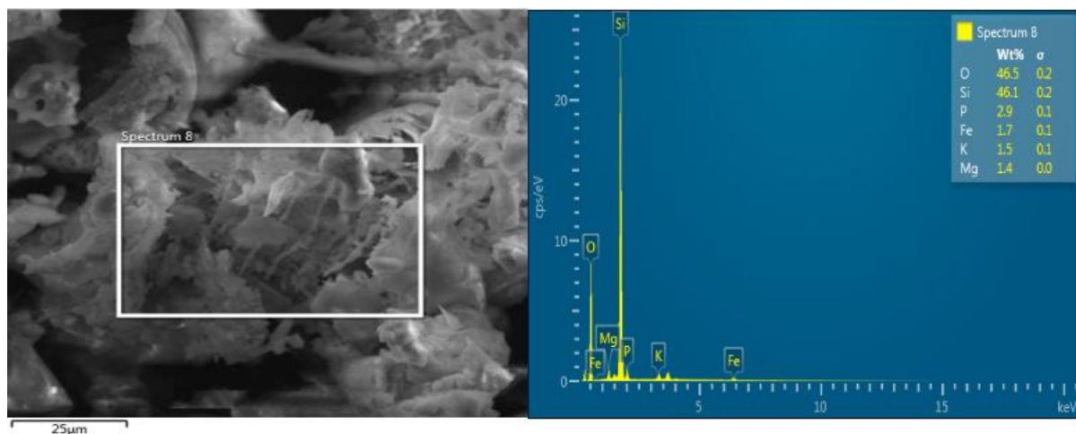
Figure 3. SEM image representative and EDX (36).
