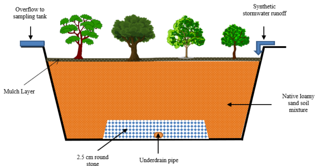
Figure 1. Layout rain garden.
