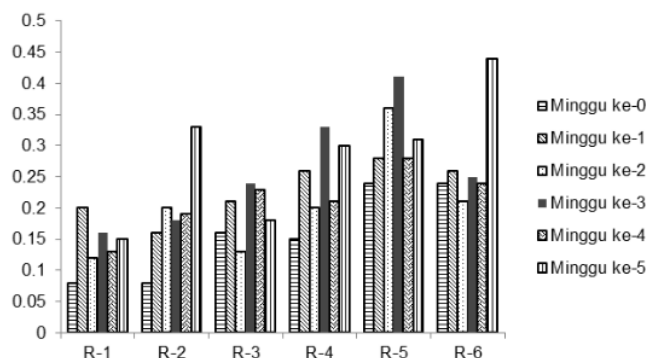
Gambar 4. Hasil Pengukuran N-Total selama Proses Composting
