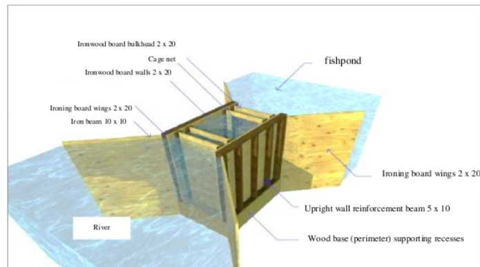
Figure 4 Typical gate at fishpond network
