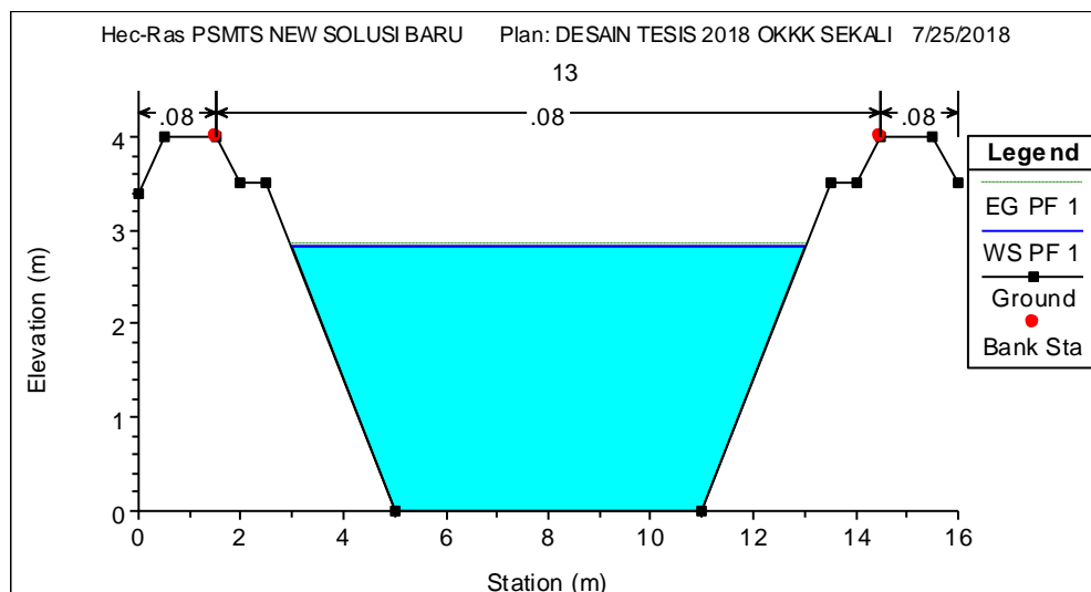
Figure 7. Cross Section Simulation P.1 SS.1-MH.1 (Source: Analysis)
