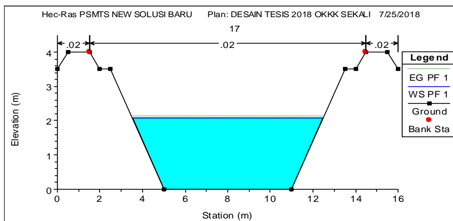
Figure 9. Cross Section Simulation P.18 SS.3-MH.3 (Source: Analysis)
