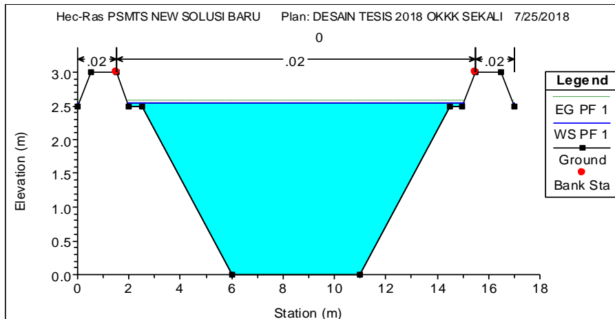
Figure 8. Cross Section Section P.5 SS.2-MH.2 (Source: Analysis)
