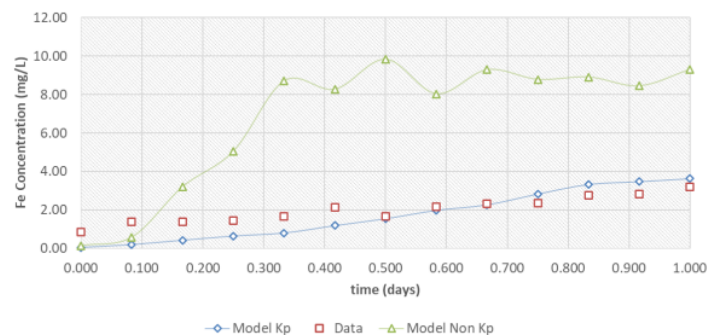
Figure 5. Model Comparison
