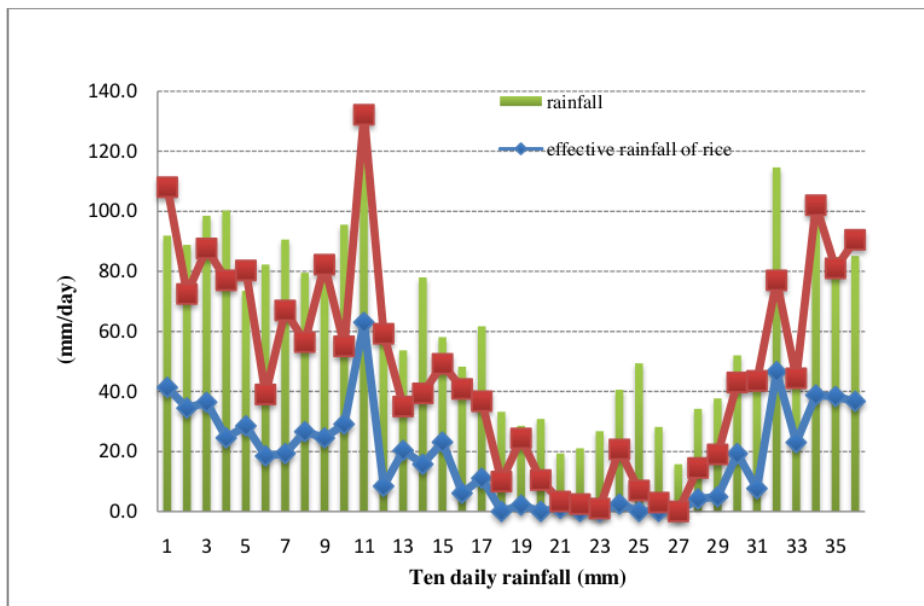
Fig.1. Relationship between effective rainfall of rice and palawija and ten daily rainfall
