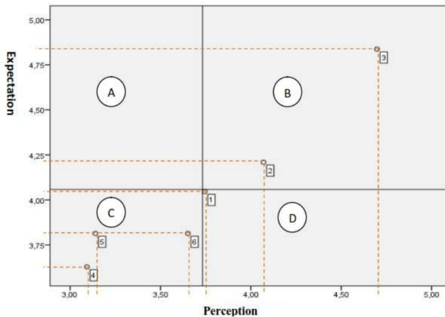
Picture. 1 Cartesian Quadrant Diagram
