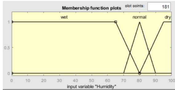
Figure 6. Humidity membership value
