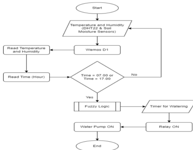
Figure 3 . System Workflow
