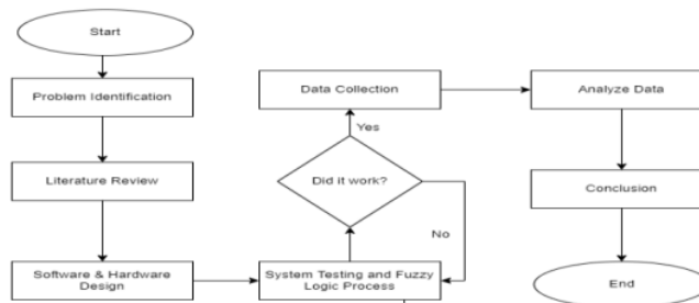
Figure 2. Research Flow
