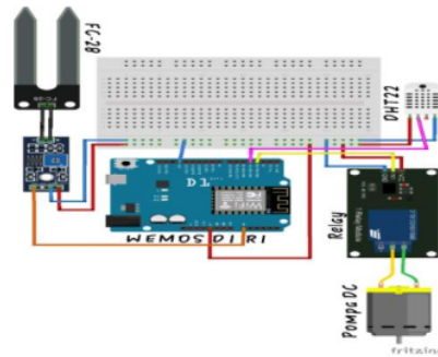
Figure 4. Hardware Circuit Wiring
