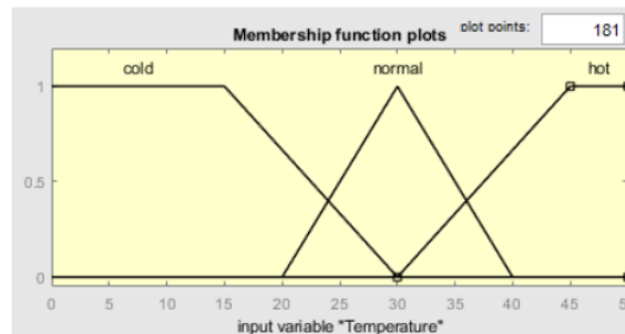
Figure 5. Temperature membership value
