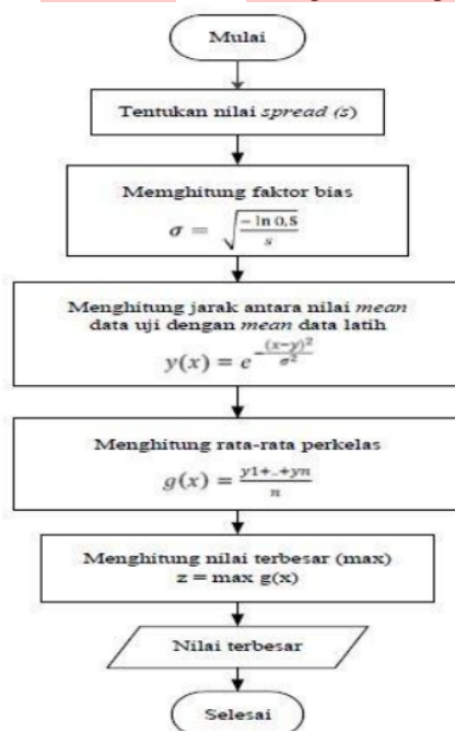
Gambar 1. Alur metode Probabilistic Neural Network (PNN)
