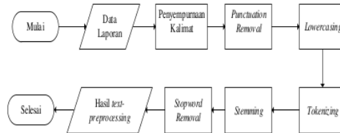
Gambar 3. Alur Text Pre-Processing
