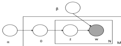
Gambar 4. Grafik representasi model probabilistik LDA
