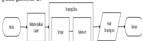
Gambar 2. Alur scraping data
