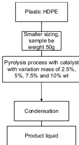
Figure 1. Flowchart of Experimental Oriented
