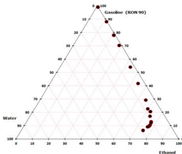
Figure 1. Triangular graphs of gasoline (RON 90)-ethanol-water under atmospheric condition
