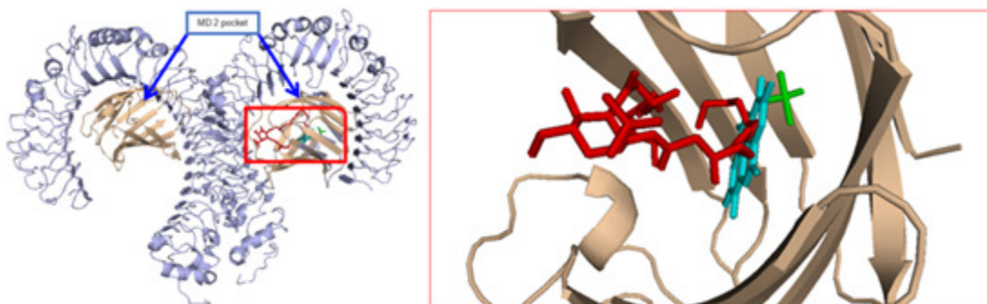
Fig. 3 : Interaction of molecular docking between the TLR4-MD2 (wheat; cartoon) with LP5 (control) (red; line), calcium phosphate (green; line) and ellagic acid (cyan; line)
