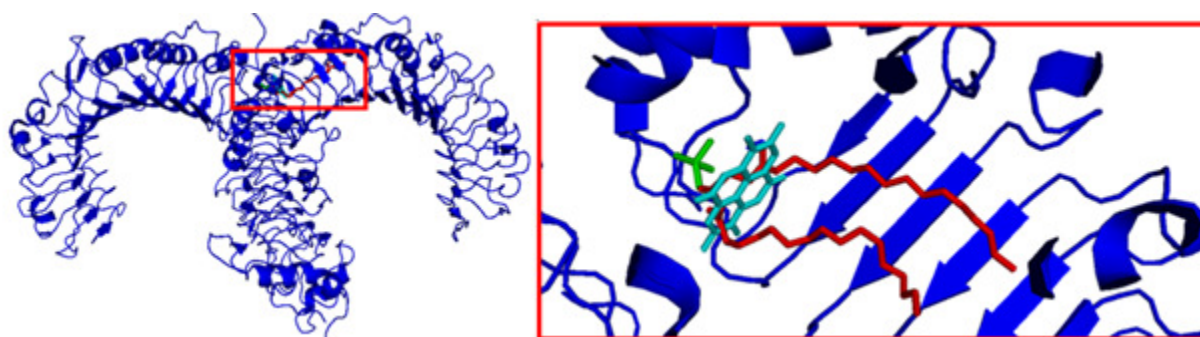
Fig. 4 : The interaction of molecular docking between TLR2 / TLR6 (blue; cartoon) with PXS (control) (red; line), calcium phosphate (green; line) and ellagic acid (cyan; line).
