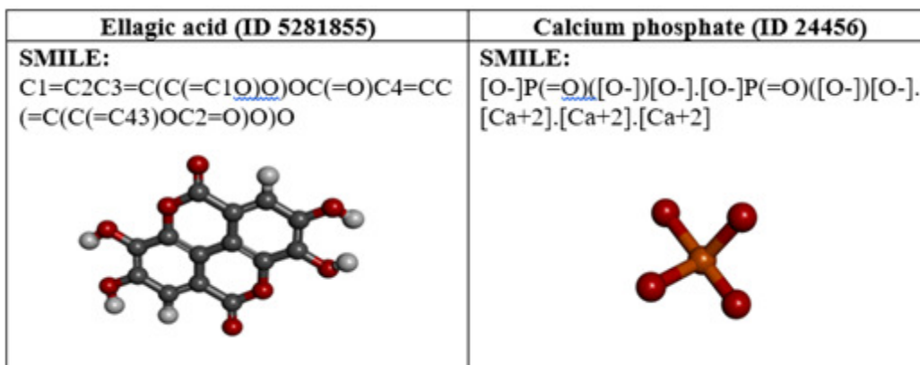
Fig. 2 : 3D structure, SMILE ellagic acid and calcium phosphate.
