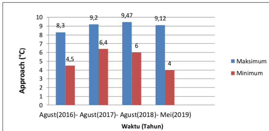
Gambar 7. Grafik Approach Cooling Tower
