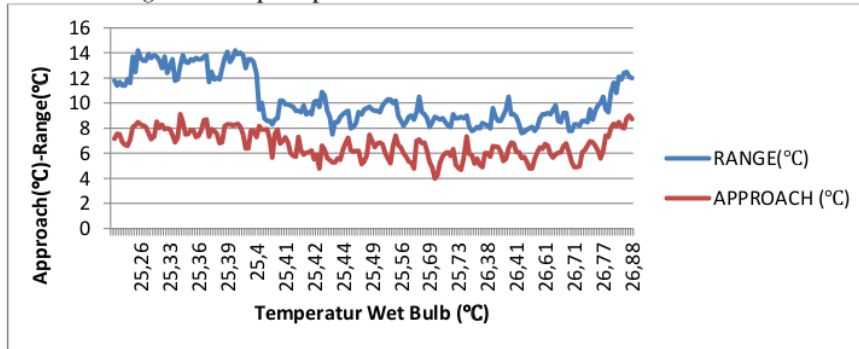
Gambar 3. Grafik Kinerja Range dan Approach Cooling tower
