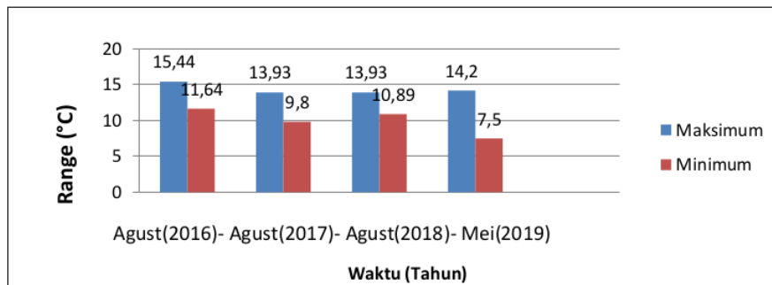
Gambar 6. Grafik Range Cooling Tower
