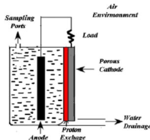
Gambar 1. Skema Single Chamber
