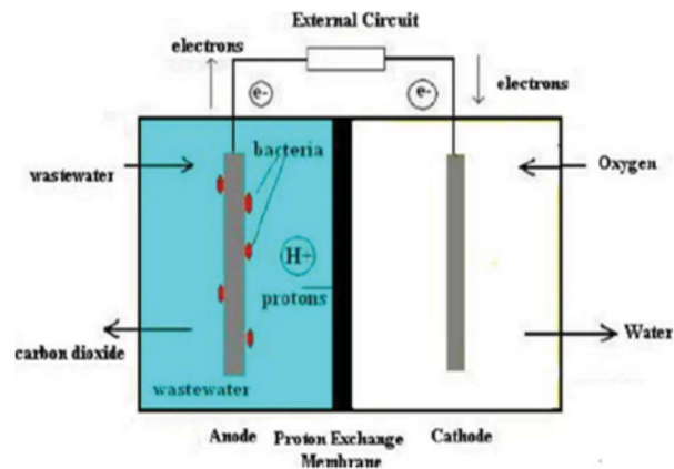
Gambar 2. Skema Dual Chamber
