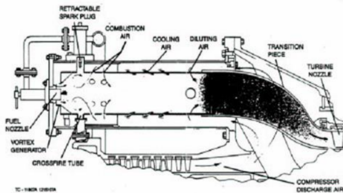
Gambar 5. Combustion Section
