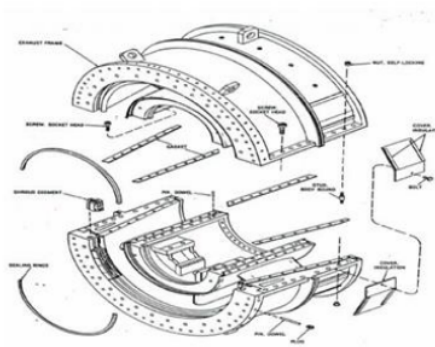
Gambar 7. Exhaust Section
