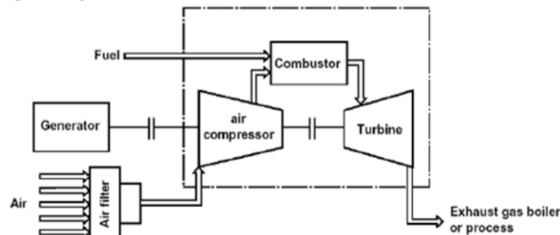
Gambar 1. Diagram Alir Turbin Gas
