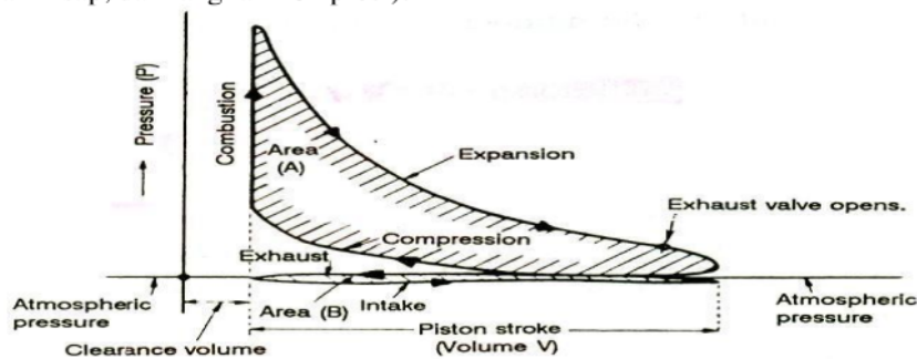
Gambar 1. Diagram Indikator Horsepower
