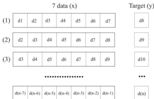
Fig. 7. Series Data Illustration
