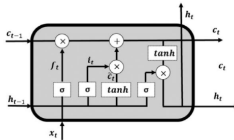
Fig. 6. LSTM Architecture
