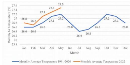
Fig. 1. Air Temperature 1991-2020 and Monthly Air Temperature 2022 Comparison
