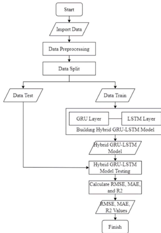
Fig. 4. Model Workflow
