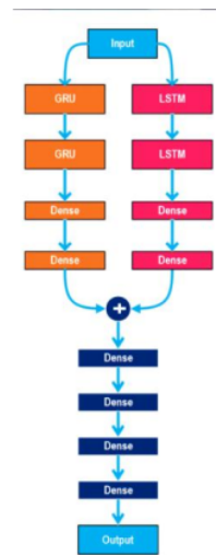
Fig. 8. Hybrid GRU-LSTM Model Architecture
