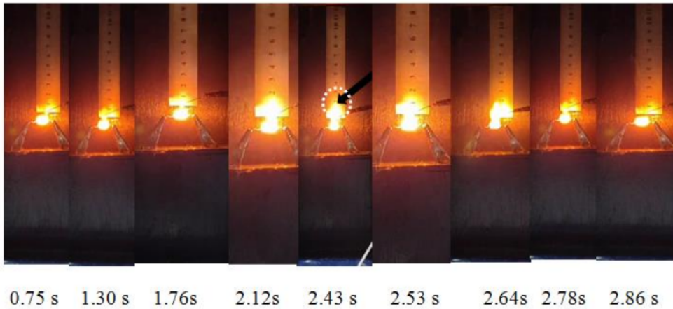
Figure 11 Visualization of Flame Percentage of 40% Methanol Mixture
