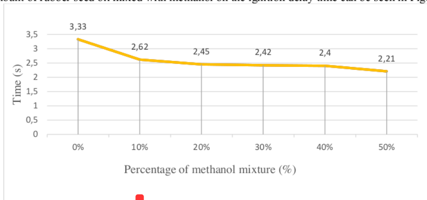
Figure 4. The influence of the percentage of the mixture of rubber seed oil with methanol on ignition delay time
