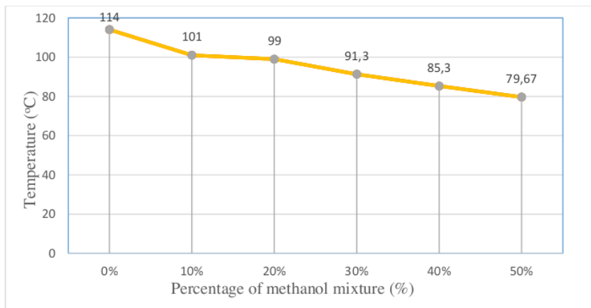
Figure 3. The effect of the amount of rubber seed oil mixed with methanol on the Flashpoint
