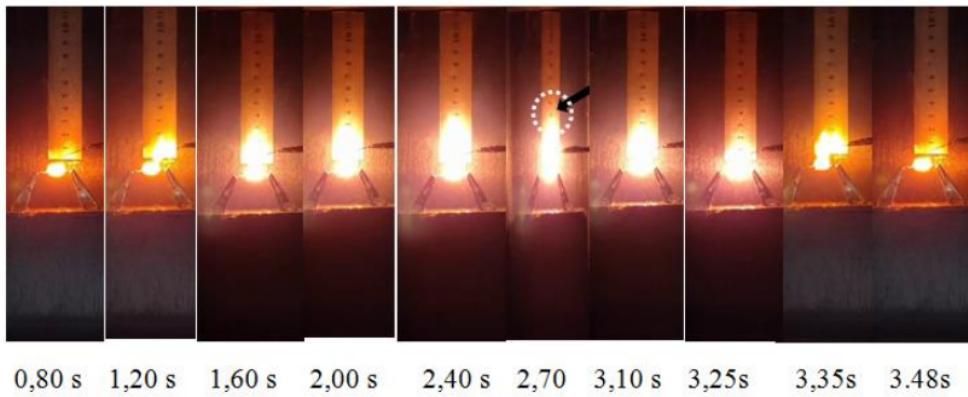
Figure 8. Visualization of Fire Mixed percentage 10%
