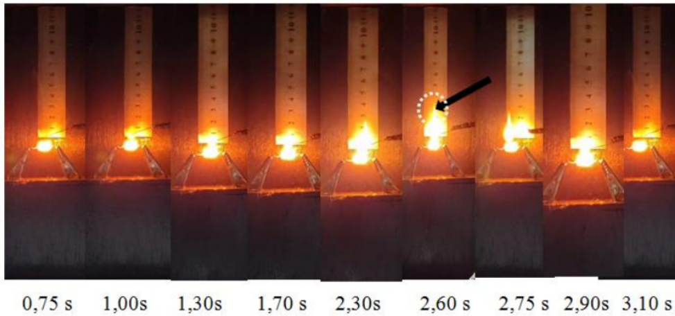
Figure 9. Visualization of Flame Percentage of Methanol Mixture 20%
