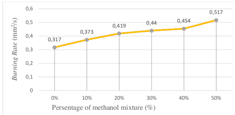
Figure 5. The effect of a mixture of methanol and rubber seed oil on the burning rate
