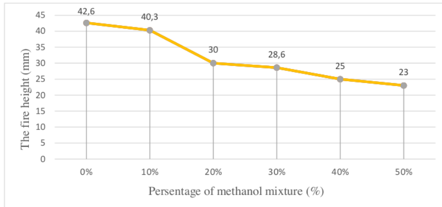
Figure 6. The effect of a mixture of rubber seed oil and methanol on fire height
