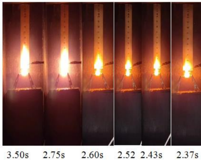
Figure 13. Comparison of Maximum Fire Height in Each Mixture With Percentages of 0%, 10%, 20%, 30%, 40%, and 50%
