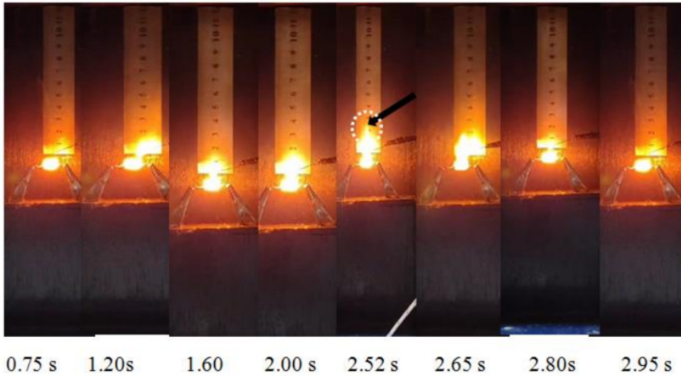
Figure 10. Visualization of Flame Percentage of 30% Methanol Mixture
