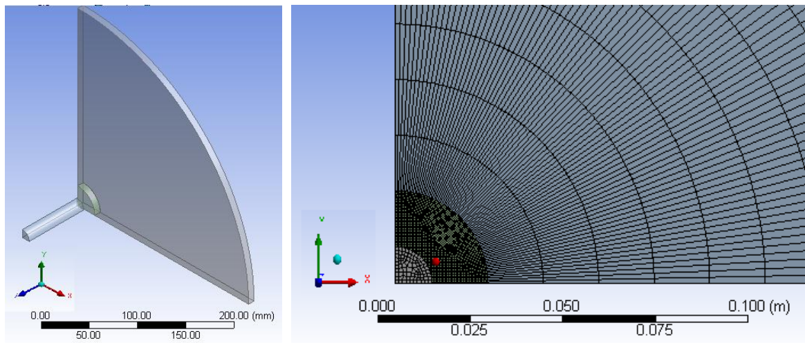
Figure 1. Modelling and meshing
