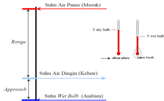
Gambar 4. Range dan Approach Cooling tower
