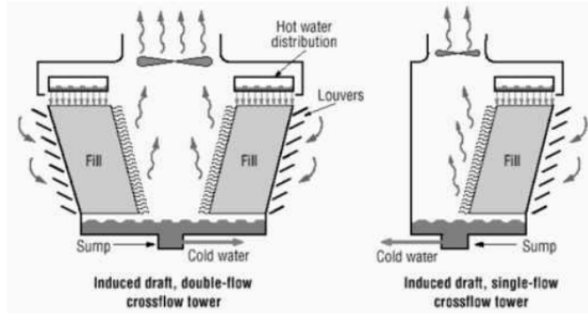
Gambar 3. Induced Draft Cooling Tower Aliran Cross-flow
