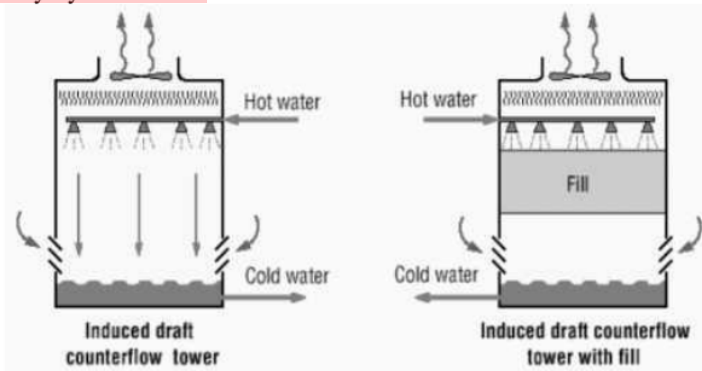
Gambar 2. Induced Draft Cooling Tower Aliran Counter-flow
