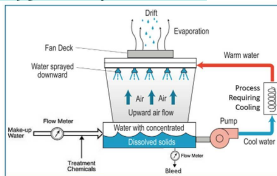
Gambar 1. Diagram Skematika Cooling tower
