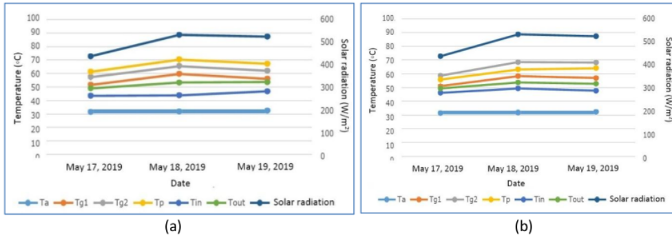
Figure 6. The relationship between average temperature and solar radiation intensity at angle of 30° (a) 5 mm glass; (b) 3 mm glass
