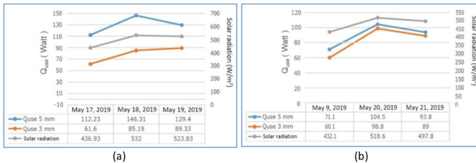
Figure 9. The relationship between average Q_{use} and solar radiation intensity of 5 mm glass and 3 mm (a) angle of 30^\circ ; (b) angle of 20^\circ
