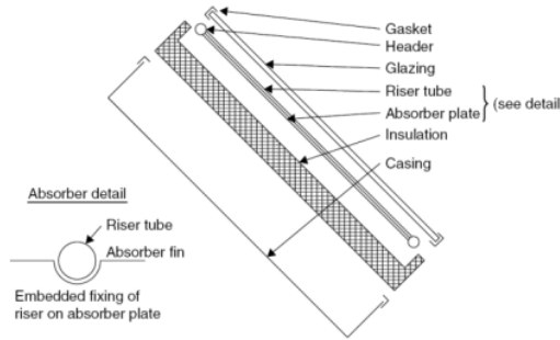
Figure 1. A flat-plate collectors and absorber details [5]
