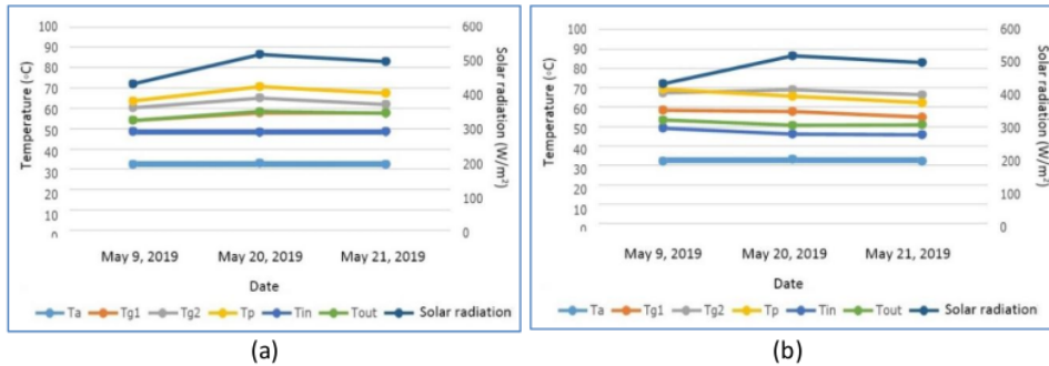
Figure 7. The relationship between average temperature and solar radiation intensity at angle of 20° (a) 5 mm glass; (b) 3 mm glass
