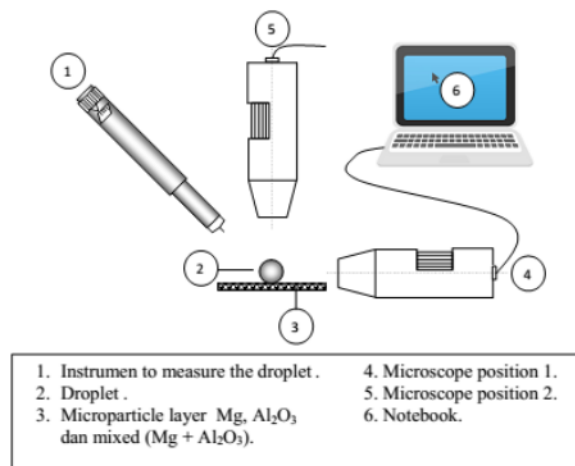
Fig. 4. Droplet contact angle measurement technique
