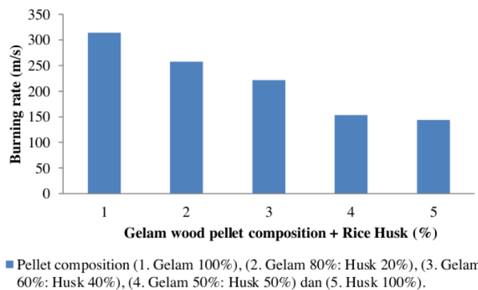
Figure 2. Graph of the Burning Rate of wood pellets for rice husks
