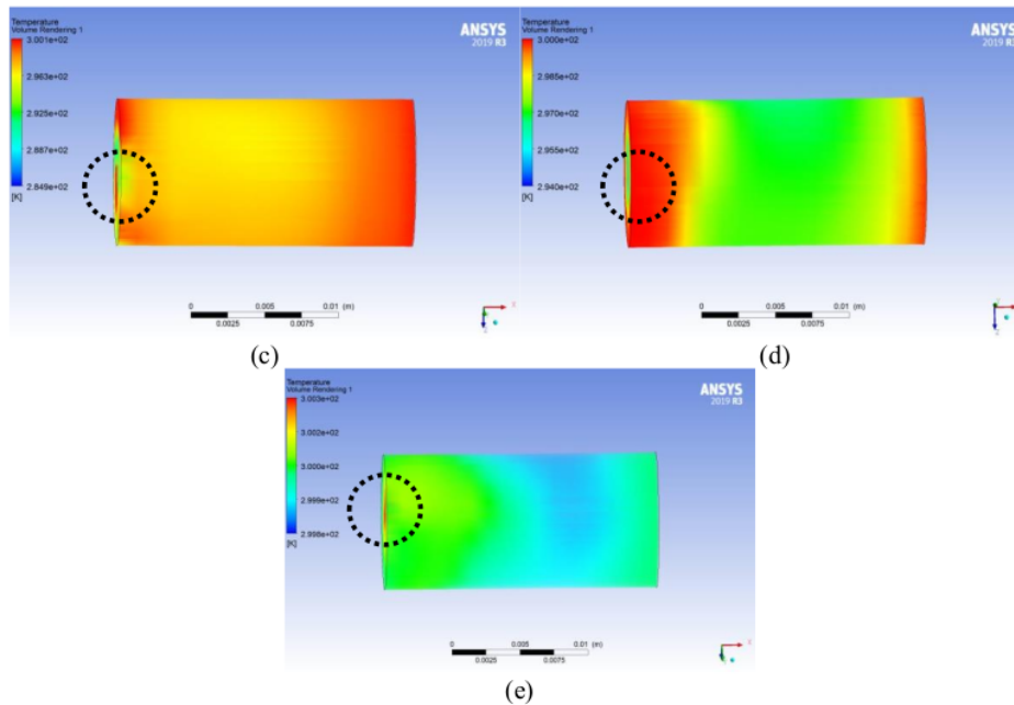
Figure 4. The results of the ANSYS simulation of pellet combustion temperature in the variation of the mixture (gelam wood + rice husk): (a). 100% gelam composition, (b). Gelam composition 80%: Rice husk 20%, (c). 60% Gelam Composition: 40% Husk, (d) 50% Gelam Composition: 50% Husk and (e). 100% Husk Composition
