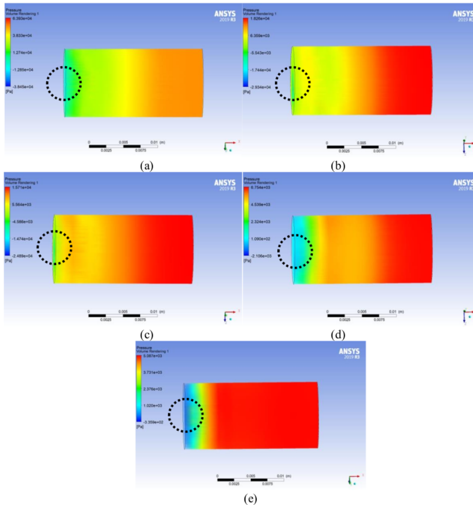
Figure 6. Simulation results of ANSYS Combustion pressure on the variation of the mixture (gelam wood + rice husk): (a). 100% gelam composition, (b). Gelam composition 80%: Rice husk 20%, (c). 60% Gelam Composition: 40% Husk, (d) 50% Glam Composition: 50% Husk and (e). 100% Husk Composition
