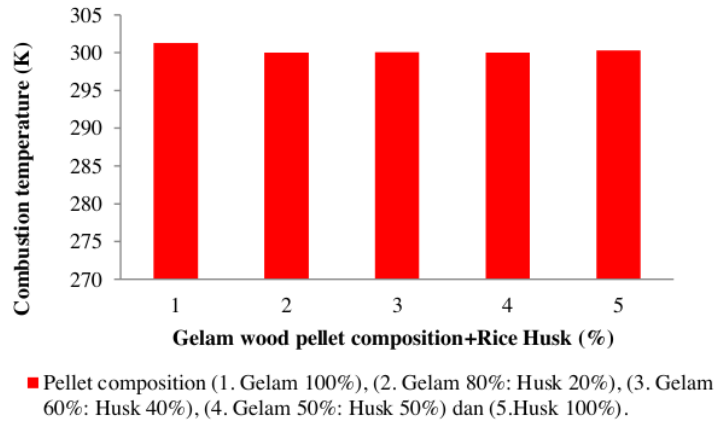
Figure 1. Graph of Burning Temperature of wood pellets for rice husks
