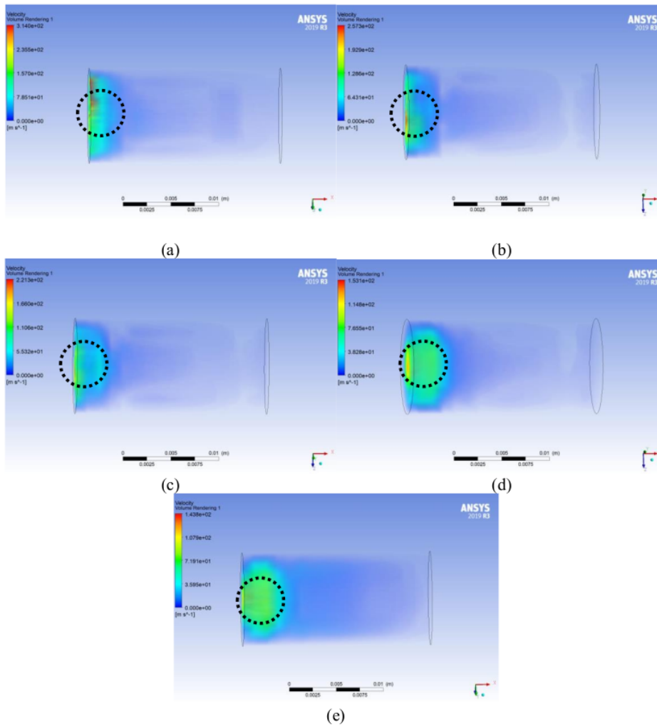
Figure 5. The results of the ANSYS simulation of the burning pellet rate in the variation of the mixture (gelam wood + rice husk): (a). 100% gelam composition, (b). Gelam composition 80%: Rice husk 20%, (c). 60% Gelam Composition: 40% Husk, (d) 50% Glam Composition: 50% Husk and (e). 100% Husk Composition
