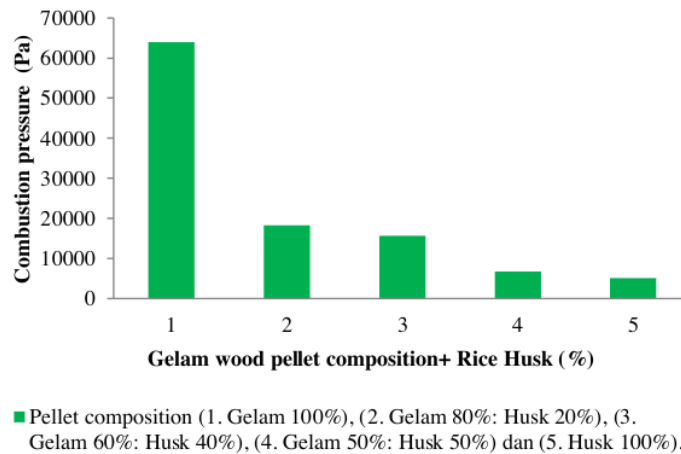
Figure 3. Graph of the Combustion Pressure of the wood-husk wood pellets
