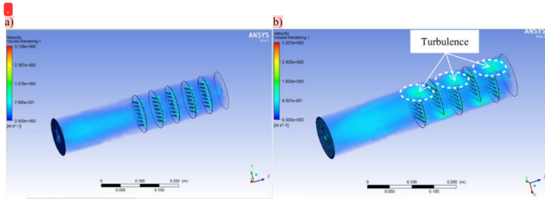
Fig. 3. The exhaust gas flow pattern passes through 5 filters at: a) Filter-not-cut type and b) Filter-cut type
