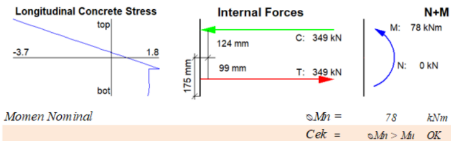
Gambar 6. Nilai Momen Nominal, M_n = 78 \text{ kNm}
