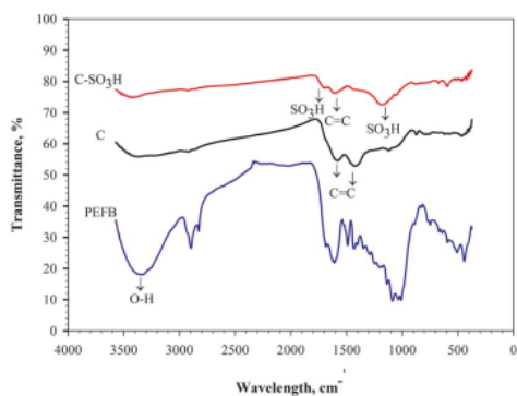
Fig. 5 FT-IR spectra of PEFB, C and C-SO 3 H.
