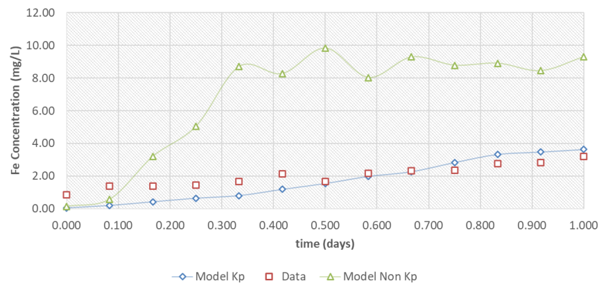
Figure 5. Model Comparison
