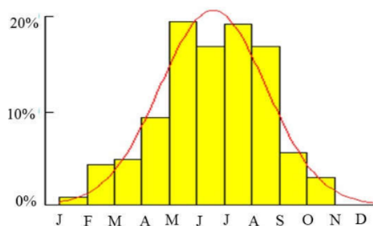
Figure 5 Labangka red spiny lobster annual recruitment pattern. Based on the recruitment pattern, it is estimated / suspected lobster spawned throughout the year, and only one peak spawning season in a year. This is based on the recruitment peak pattern that occurs which means that in that month the lobster population is relatively abundant and exploited. This situation is relevant to Effendie's statement (2002) that recruitment is the addition of new individuals into the fishery resources stock caught by fishing gear. The addition of new individual fish resources in a waters area for each size class is very closely related to environmental conditions (Dodds, 2002)
