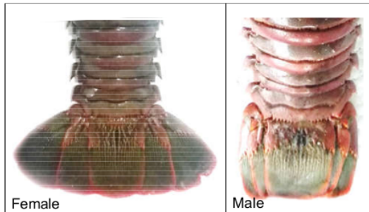
Figure 3 Female and male uropod of P. penicillatus
