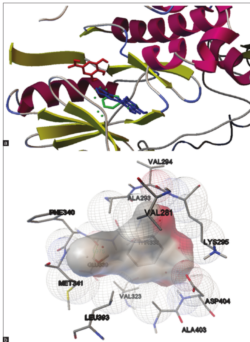
Figure 6: Comparison of the ligand position between cocystal ligand (blue), gallic acid (red), and methyl gallate (green) on 2HCK receptor (a); and interaction between receptor protein and methyl gallate (b)
