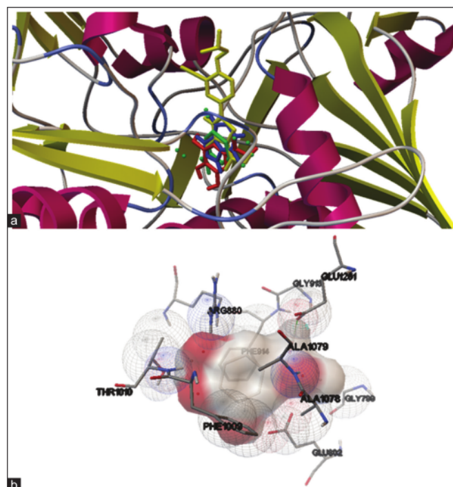
Figure 4: Comparison of the ligand position between cocystal ligand (blue), febusostat (yellow), gallic acid (red), and methyl gallate (green) on 3NRZ receptor (a); and interaction between receptor protein and methyl gallate (b)
