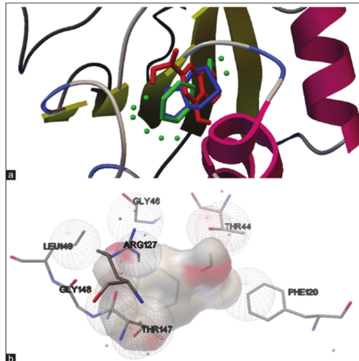
Figure 3: Comparison of the ligand position between cocystal ligand (blue), gallic acid (red), and methyl gallate (green) on 3MNG receptor (a); and interaction between receptor protein and methyl gallate (b)
