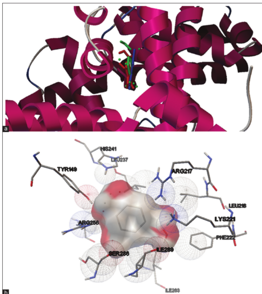
Figure 5: Comparison of the ligand position between cocrystal ligand (blue), gallic acid (red), and methyl gallate (green) on 4JK4 receptor (a); and interaction between receptor protein and methyl gallate (b)
