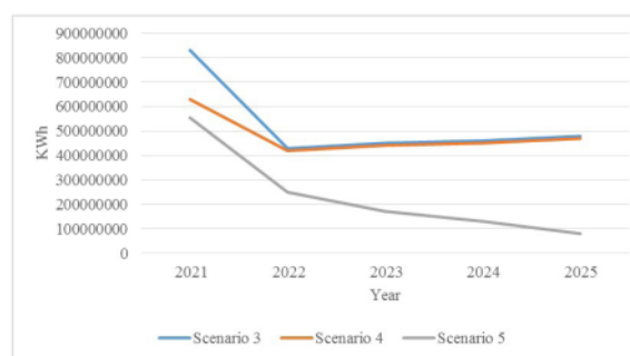
Figure 1. Power consumption for water pumping in scenarios 3, 4, and 5.
