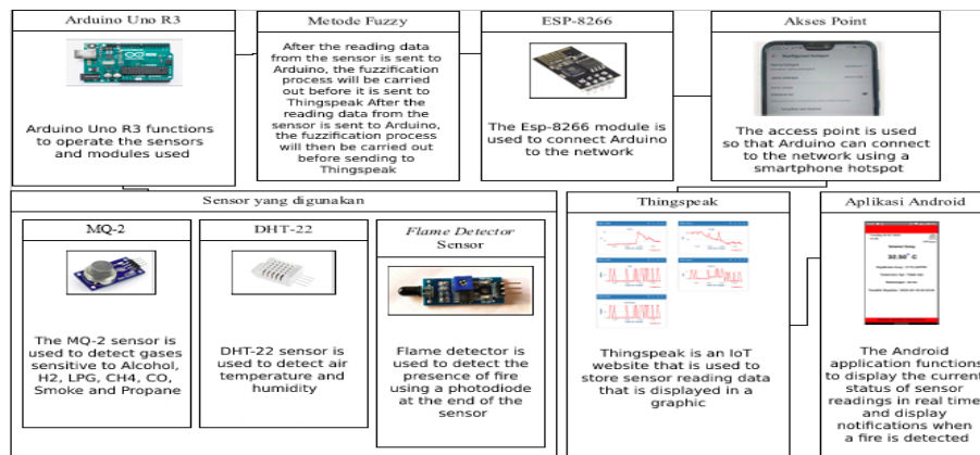
Figure 2. General Description of the System
