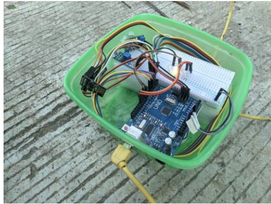
Figure 12. Sensor Circuit Above Breadboard
