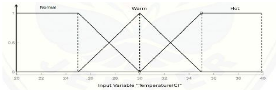
Figure 4. List of Temperature Membership
