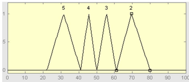
Fig. 8. Fuzzy Membership Function for Value
