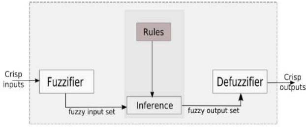
Fig. 5. Fuzzy Component
