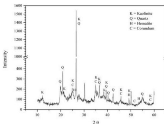
Fig. 1 XRD pattern of WTS
