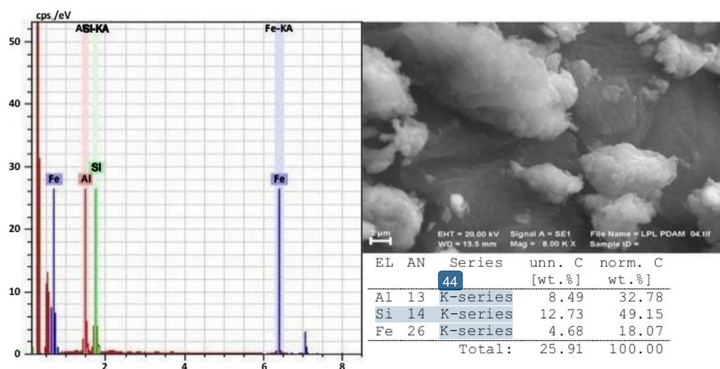
Fig. 2 SEM pictures of WTS
