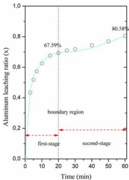
Fig. 7 Division of stages in Al leaching process
