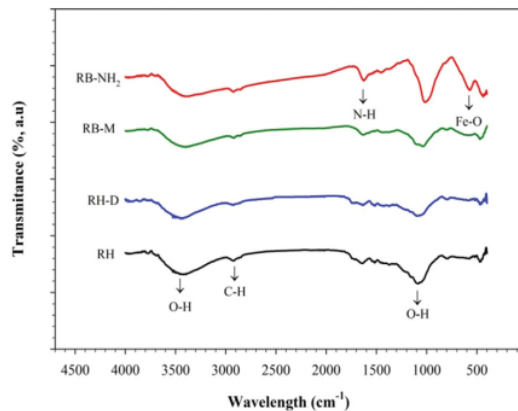
Fig. 3. FT-IR Spectra of rice husk (RH), RH after delignification (RH-D), rice husk magnetic biocomposite without amine (RB-M), and amine rice husk magnetic biocomposite (RB-NH 2 ).
