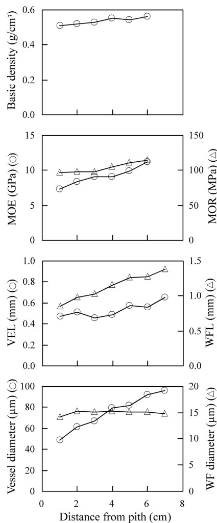
Fig. 4. Radial variations of basic density, static bending properties, cell length, and cell diameter in kayu manis.
