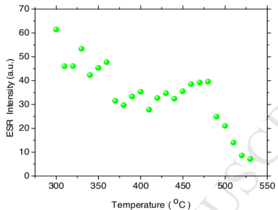
7 Fig. 8. Thermal annealing behaviour of center IV in \text{CaAl}_{12}\text{O}_{19}:\text{Ho} phosphor.
