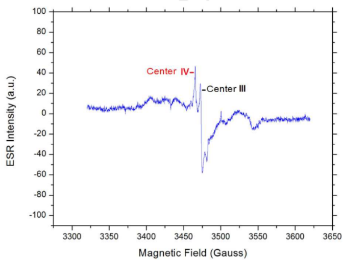
Fig. 9 Room temperature ESR spectrum of irradiated \text{CaAl}_{12}\text{O}_{19}:\text{Ho} phosphor (gamma dose: 10 kGy) after warming to 200 °C at a heating rate of 4 °C/S in the TL instrument
