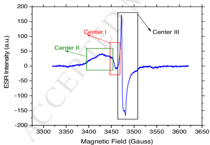
Fig. 5. (a) Room temperature ESR spectrum of irradiated \text{CaAl}_{12}\text{O}_{19}:\text{Ho} phosphor (gamma dose: 10 kGy). Line labelled as I is due to an \text{O}^{\cdot -} ion. Center II line is assigned to an \text{O}_2^{\cdot -} ion and center III is attributed to a \text{F}^+ center. (b) ESR spectrum at room temperature after warming the irradiated phosphor to 200\text{ }^{\circ}\text{C} at a heating rate of 4\text{ }^{\circ}\text{C} in the TL instrument.
