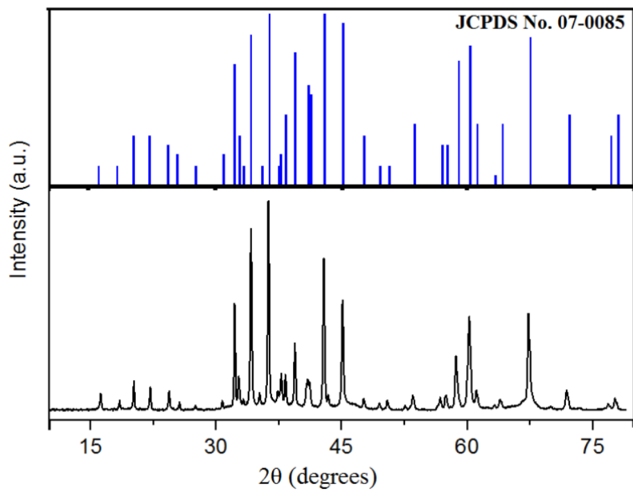
Fig. 1. Powder XRD pattern of \text{CaAl}_{12}\text{O}_{19}:\text{Ho}^{3+} phosphor prepared at 500 °C along with the standard JCPDS pattern
