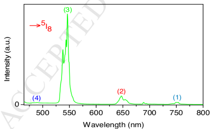
Fig. 3. (a) The transitions of the peaks are shown in energy level diagram of Ho 3+ ion, (b) excitation spectrum of CaAl 12 O 19 :Ho 3+ phosphor ( \lambda_{em} = 546 nm), and (c) Emission spectrum of CaAl 12 O 19 :Ho 3+ phosphor ( \lambda_{ex} = 450 nm).
