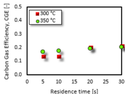
Fig.1. Effect of temperature and residence time on gasification efficiency.
