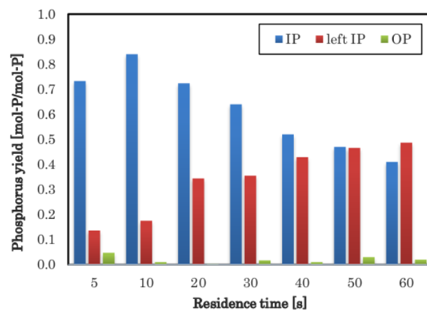
Fig.4. Effect of residence time on phosphorus behavior in SCWG of sewage sludge at 600 °C
