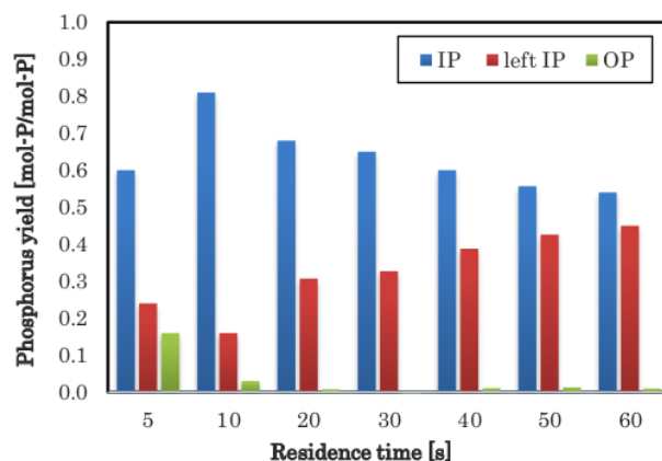
Fig.2. Effect of residence time on phosphorus behavior in SCWG of sewage sludge at 500 °C
