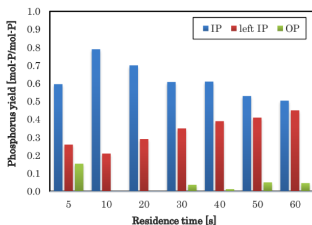
Fig.3. Effect of residence time on phosphorus behavior in SCWG of sewage sludge at 550 °C
