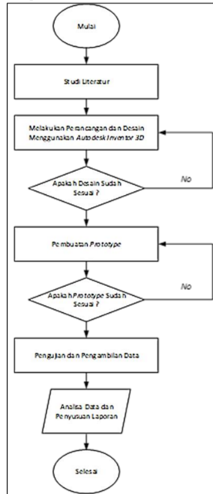
Gambar 1. Diagram Alir
