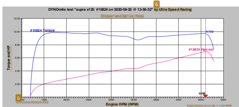
Gambar 4. Performance mesin tanpa adsorben
