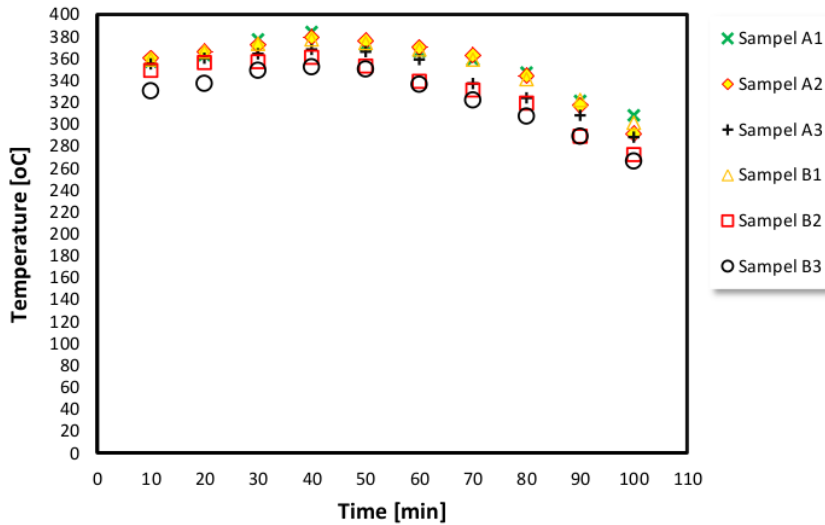
Figure 1. Temperature profile of the briquettes sample
