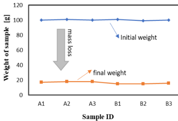
Figure 2. Mass loss of briquette sample
