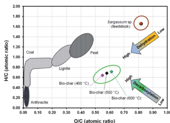
Fig. 6 Van Krevelen diagram of the biochar derived from Sargassum sp. pyrolysis.
