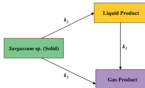
Fig. 9 Reaction pathway of macroalgae decomposition during pyrolysis.
