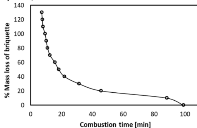
Figure 3. Combustion rate of briquette sample
