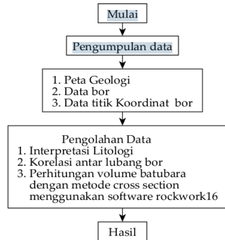
Gambar 1. Bagan Penelitian.
