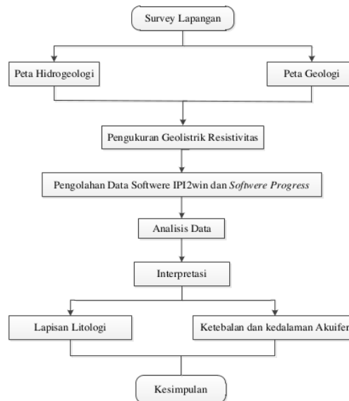
Gambar 2. Diagram alir
