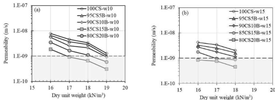
Fig. 3 Effect of density on the permeability of compacted claystone-bentonite mixtures.
